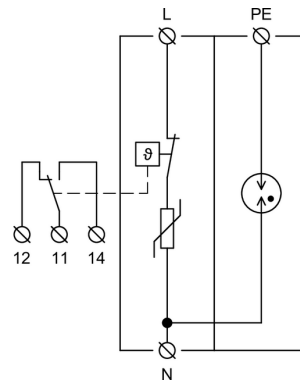
Internal diagram
