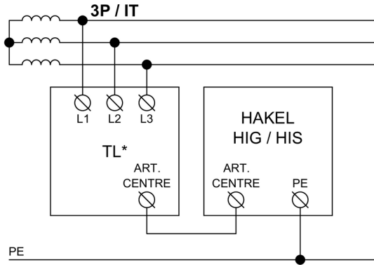
Application wiring diagram (installation)
